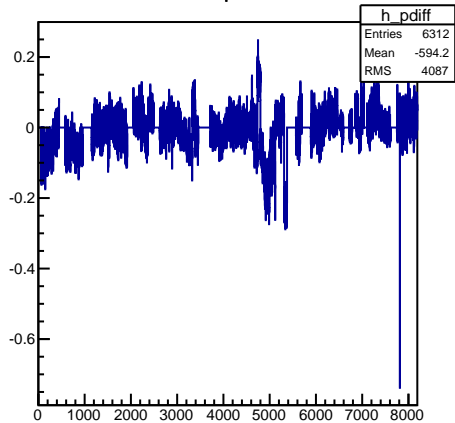
h_piff
