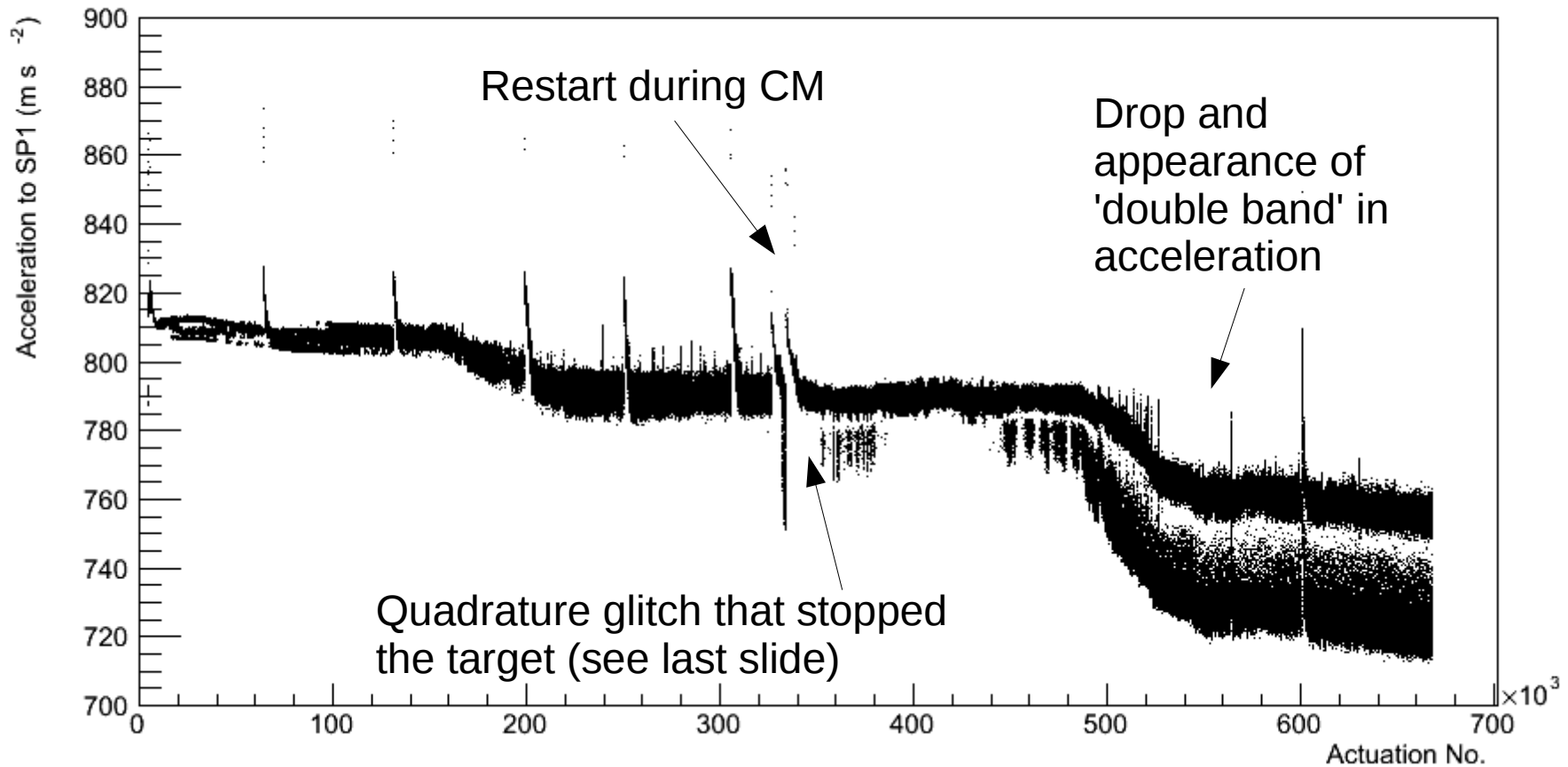
S1.1(R78) - Acceleration to SP1 ( \text{m s}^{-2} )
