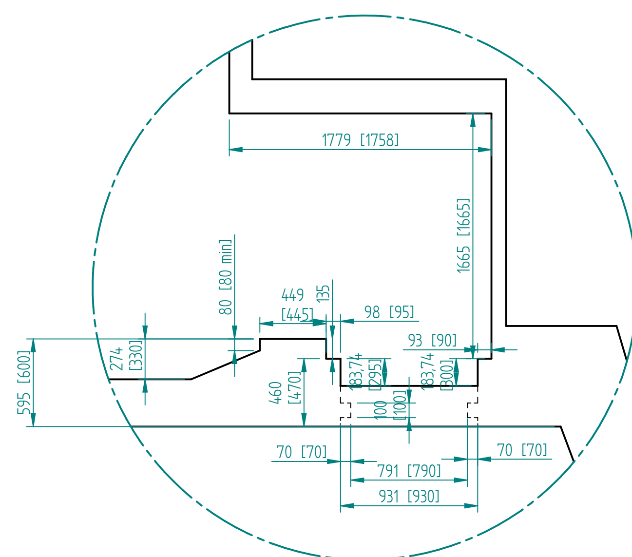
DETAIL A
